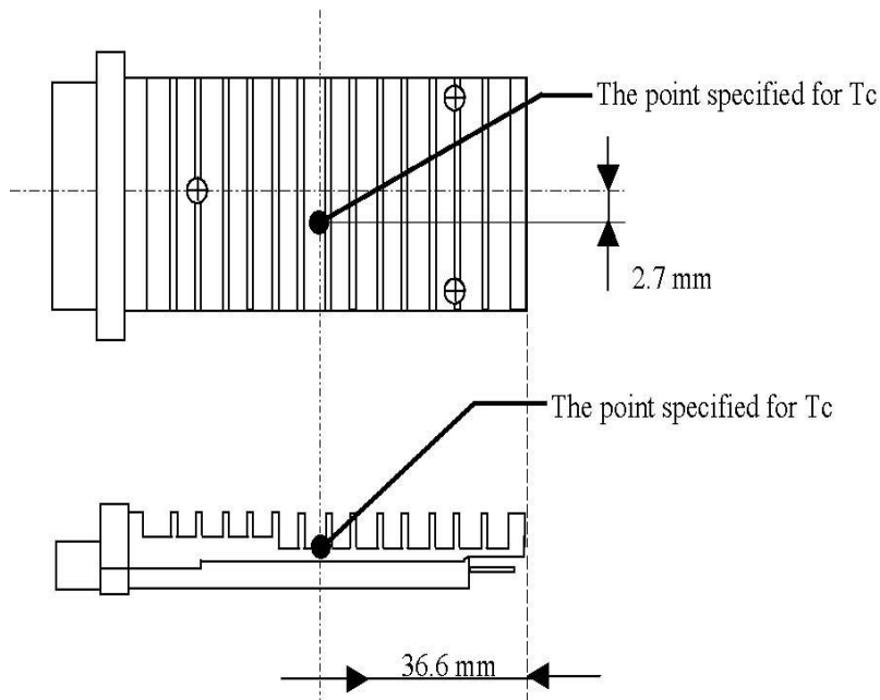
Figure 2 The Point Specified for Case Temperature (Tc)
